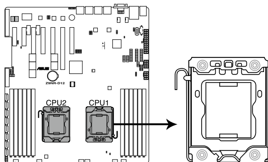
Z9NR-D12 CPU LGA1356 Socket
