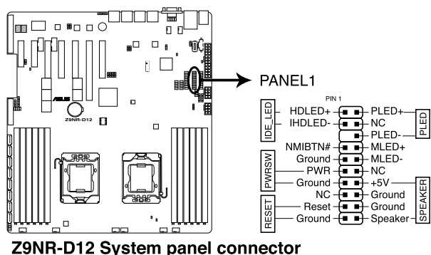
Z9NR-D12 System panel connector
