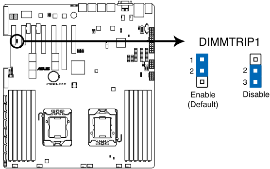
Z9NR-D12 DIMM Thermaltrip setting
