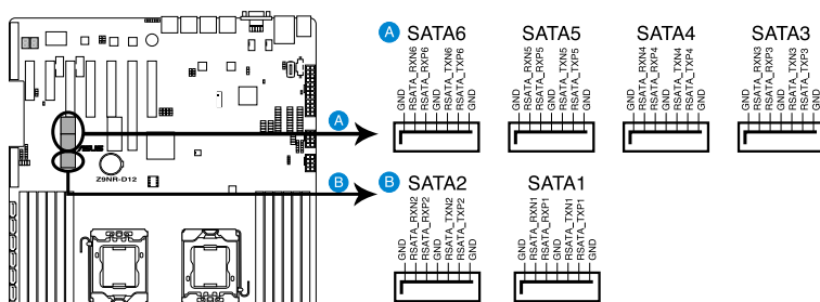
Z9NR-D12 SATA connectors
