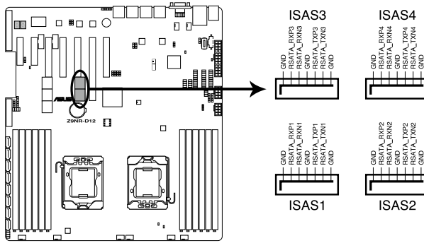
Z9NR-D12 SATA connectors (SCU)
