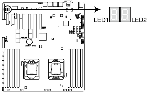
Z9NR-D12 Q-Code LED
