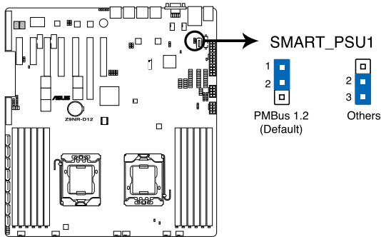
Z9NR-D12 PMBus 1.2 PSU setting
