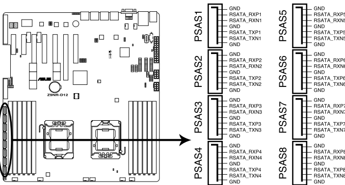
Z9NR-D12 PSAS connectors
