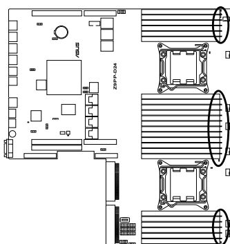
Z9PP-D24 ERR DIMM LED
