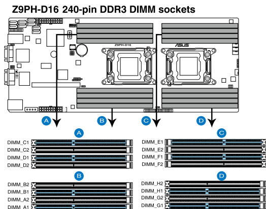
Z9PH-D16/FDR and QDR 240-pin DDR3 DIMM sockets
