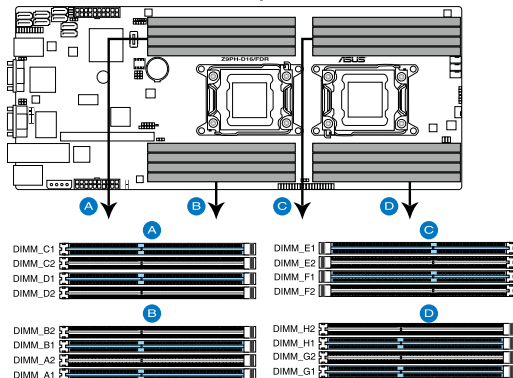
Z9PH-D16/FDR and QDR 240-pin DDR3 DIMM sockets
