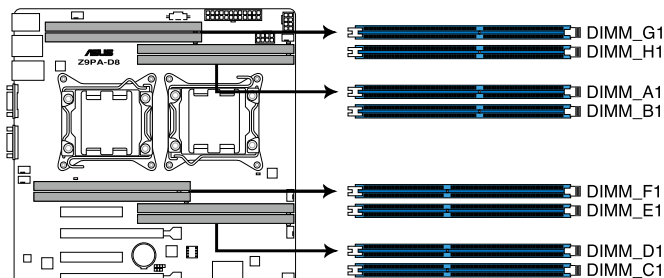
Z9PA-D8 240-pin DDR3 DIMM sockets
